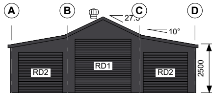
ELEVATION GRID 1
