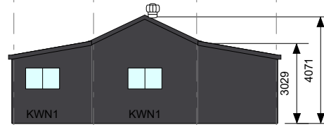
ELEVATION GRID 3
